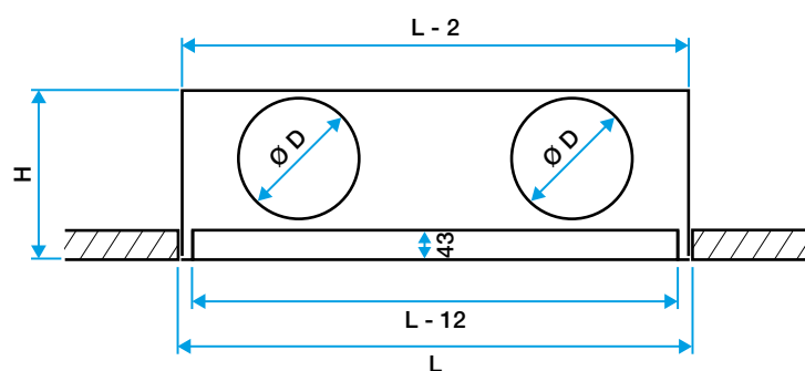
plenum LINED SLIM
