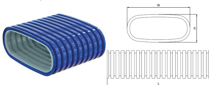
Ovale Optiflex®-buizen
