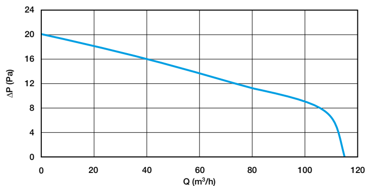
Ventilatiecurve DESIGN 125
