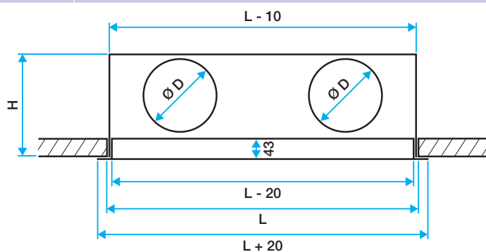
Plénum LINED
